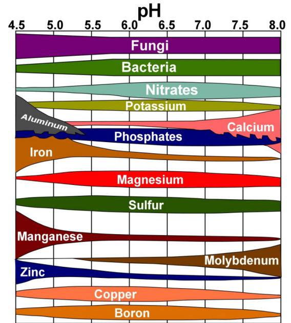
Figure 1. The availability of plant nutrients, toxic elements and microbial activity as influenced by soil pH. Wider bars indicate increased availability (activity).
